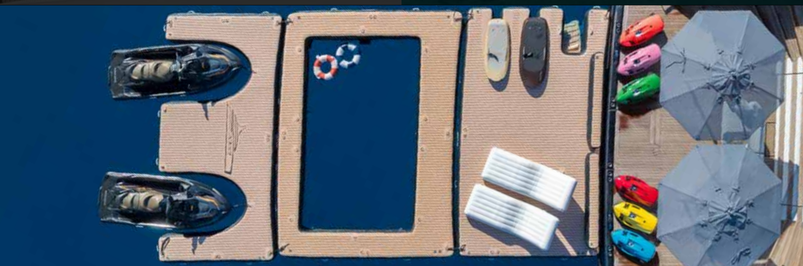
Stacking Sea Pool - each section is contoured to the swim platform, and the contour is repeated along the aft edge, allowing each element to be used independently or in any combination
